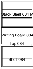
Stack Shelf 084 M + Writing Board 084 + Top 084 + Shelf 084 W84, D44, H182
