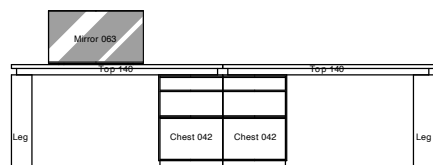
Top 140 + Top 140 + Leg + Chest 042 + Chest 042 + Leg W280. D44. H70
